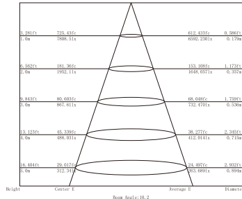
Lux Distance Curve (3000K, 10°)
