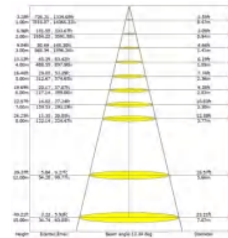
Lux Distance Curve (3000K 15X45°)
