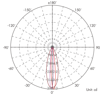
Light Distribution Curve (3000K, 10x30°)
