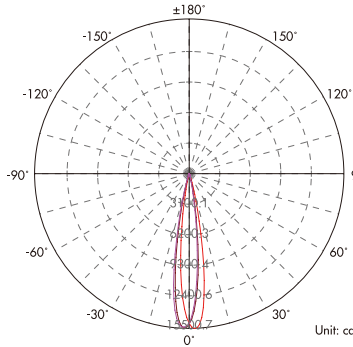
Light Distribution Curve (3000K, 1x25°)
