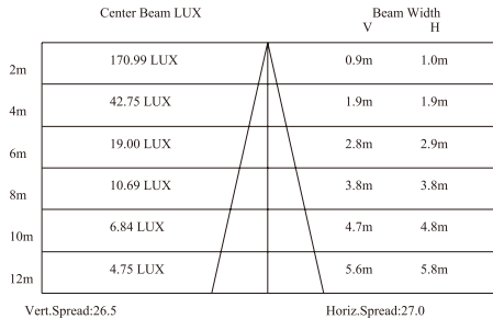
Lux Distance Curve (3000K, 1x25°)
