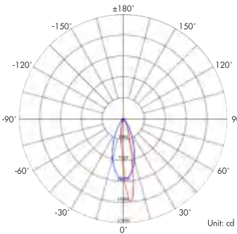
Light Distribution Curve (3000K 15X45°)
