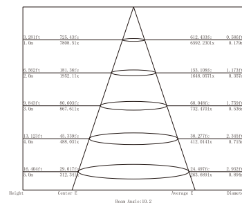
Lux Distance Curve (3000K, 10°)
