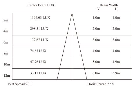
Lux Distance Curve (3000K, 1x25°)
