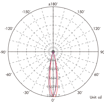
Light Distribution Curve (3000K 30°)
