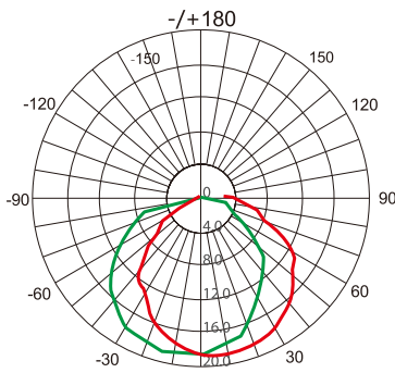
Light Distribution Curve (RGBW)
