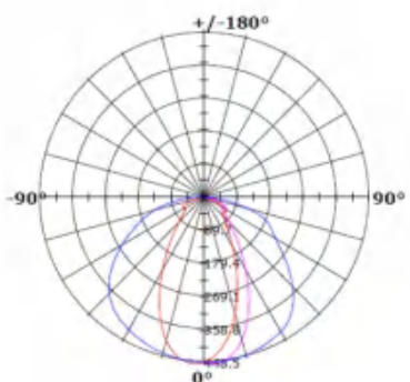
Light Distribution Curve (3000K 120°)
