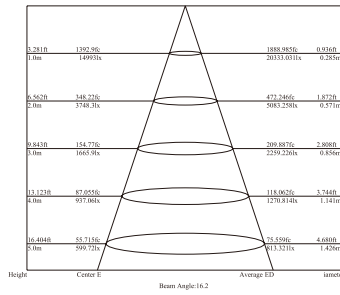
Lux Distance Curve (3000K, 1x25°)
