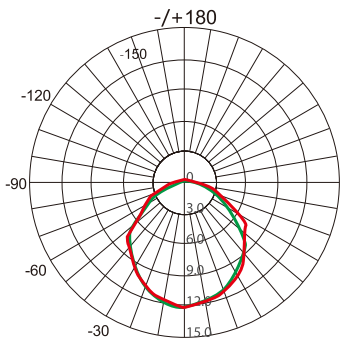
Light Distribution Curve (RGB)
