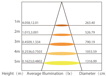
Lux Distance Curve (RGB)
