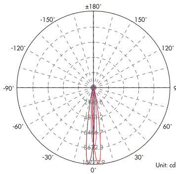
Light Distribution Curve (3000K, 10°)
