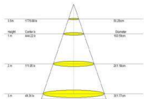
Lux Distance Curve (3000K 120°)
