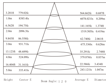
Lux Distance Curve (3000K, 1x25°)
