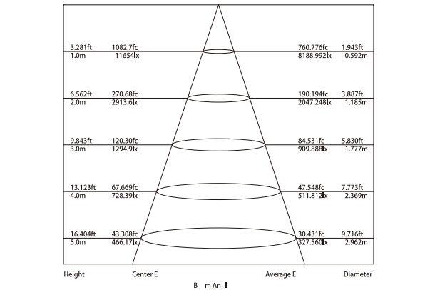
Lux Distance Curve (3000K 15°)-----
