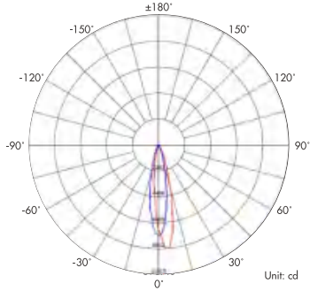
Light Distribution Curve (3000K 15X30°)
