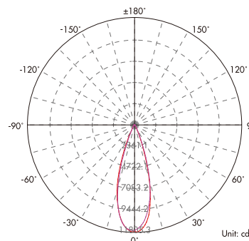
Light Distribution Curve (3000K 15°)
