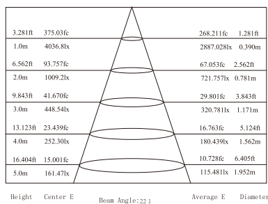
Lux Distance Curve (3000K, 1x25°)-----
