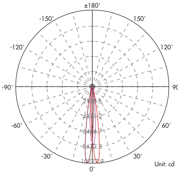
Light Distribution Curve (3000K, 10°)
