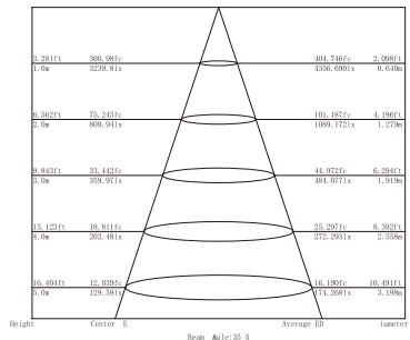
Lux Distance Curve (3000K 30°)
