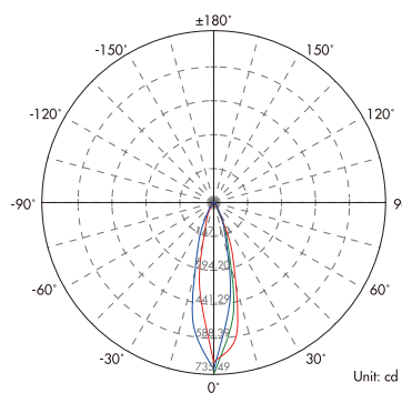
Light Distribution Curve (3000K, 1x25°).....
