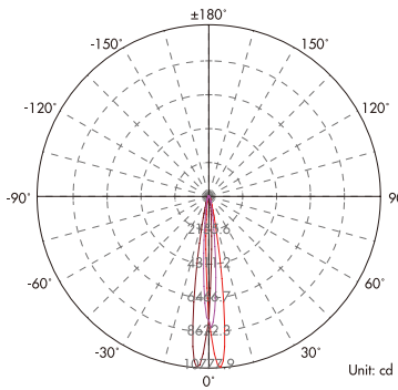
Light Distribution Curve (3000K, 10°)
