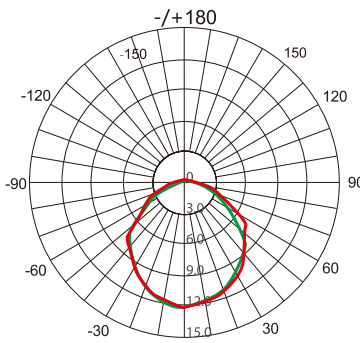
Light Distribution Curve (RGB)
