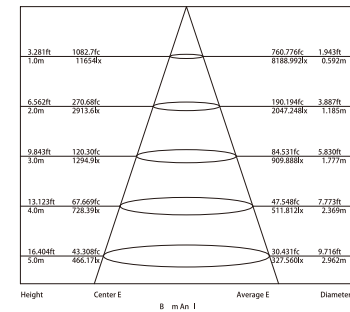
Lux Distance Curve (3000K 15°)
