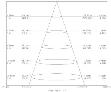
Lux Distance Curve (3000K, 10x30°)
