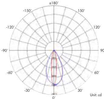
Light Distribution Curve (4000K 15X45°)
