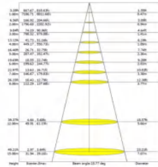
Lux Distance Curve (3000K 15X30°)
