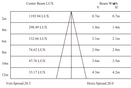
Lux Distance Curve (3000K, 1x25°)
