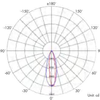
Light Distribution Curve (3000K 15X30°)
