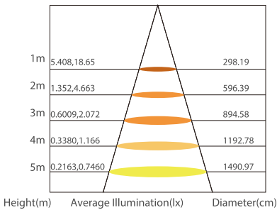
Lux Distance Curve (RGBW)
