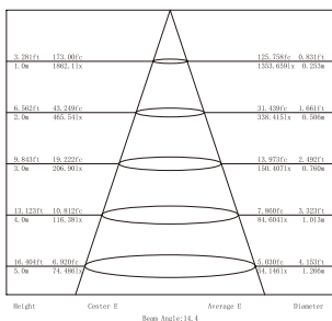
Lux Distance Curve (3000K, 1x25°)
