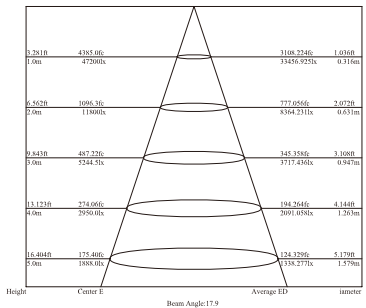
Lux Distance Curve (3000K 30°)
