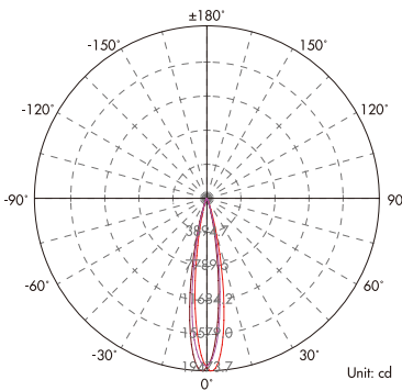
Light Distribution Curve (3000K 30°)
