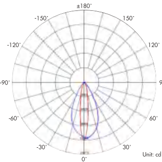
Light Distribution Curve (4000K 15X45°)
