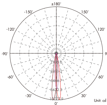
Light Distribution Curve (3000K, 10°)
