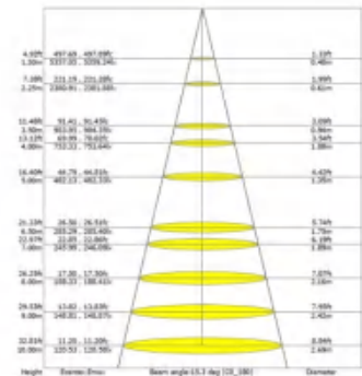
Lux Distance Curve (4000K 15X45°)
