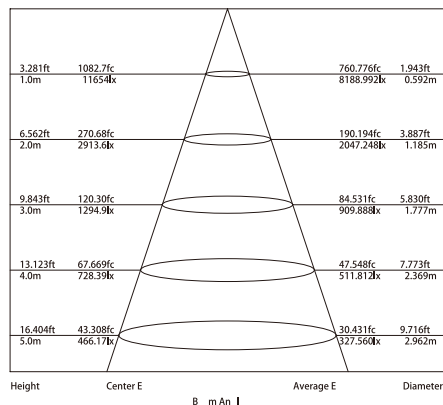
Lux Distance Curve (3000K 15°)-----
