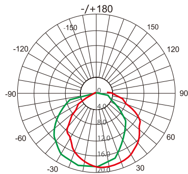
Light Distribution Curve (RGBW)
