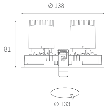
Linan Circular Edged two head
